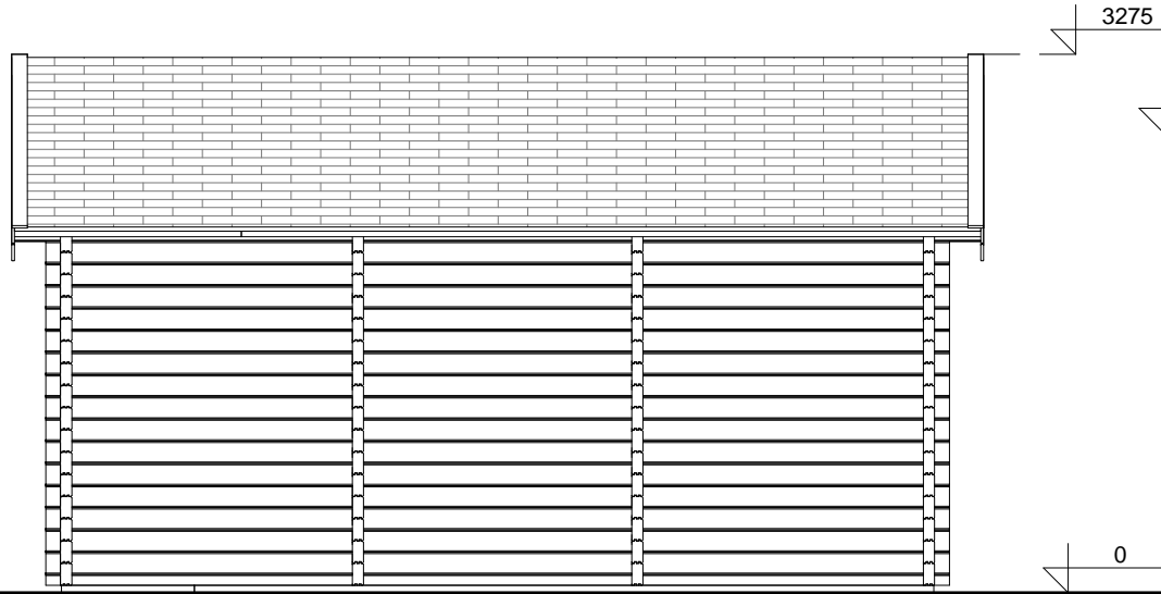
REAR VIEW
