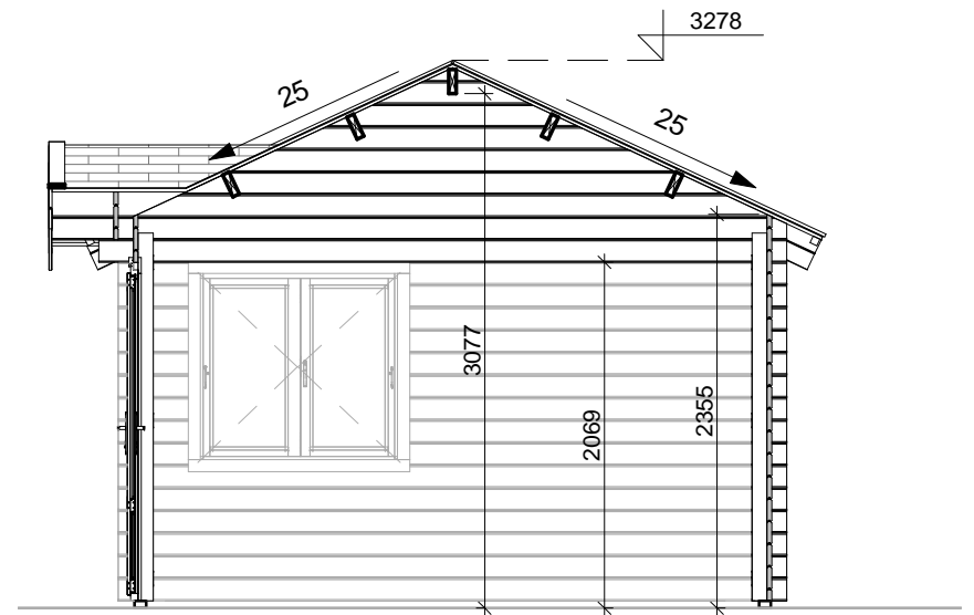
SECTION 1-1
