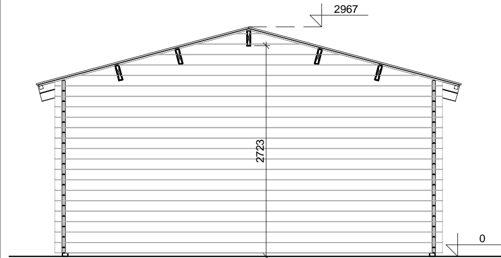
SECTION 1-1
