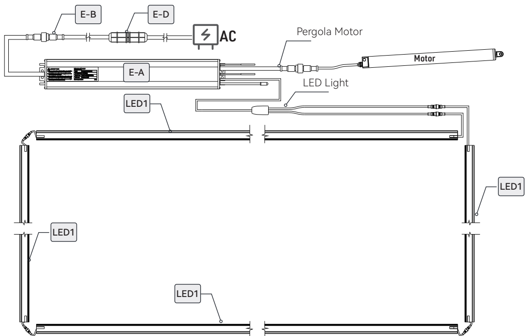
Cable Diagram
