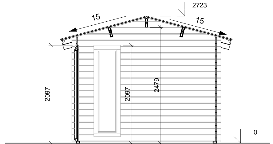
SECTION 1-1
