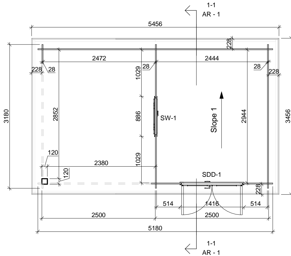
FLOOR PLAN
