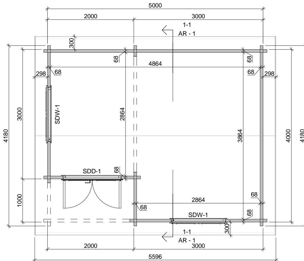
FLOOR PLAN
