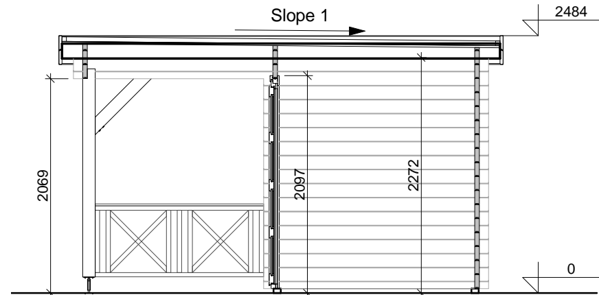
SECTION 1-1
