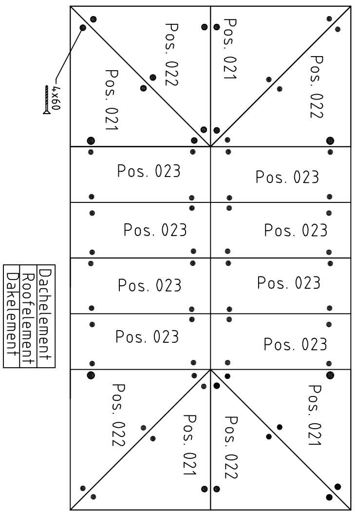
Blokhut 3030+Z 40 / 11
