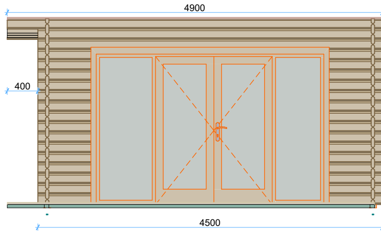
Back Elevation
