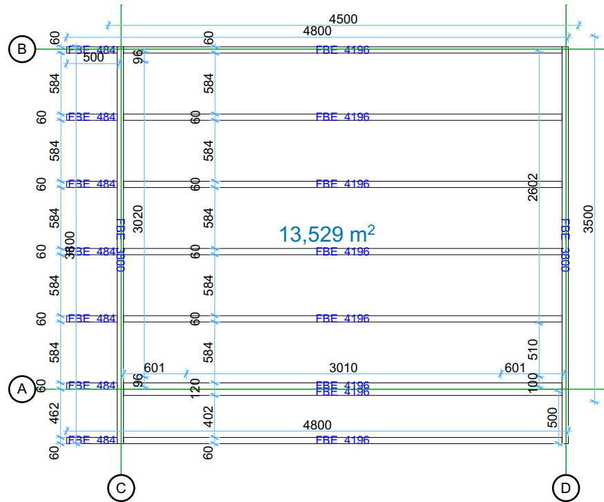
Floor bearers
