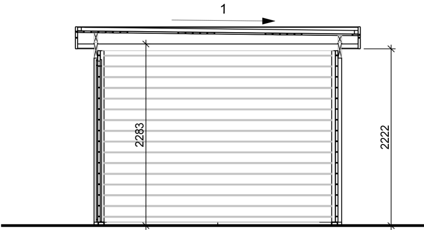
SECTION 1-1
