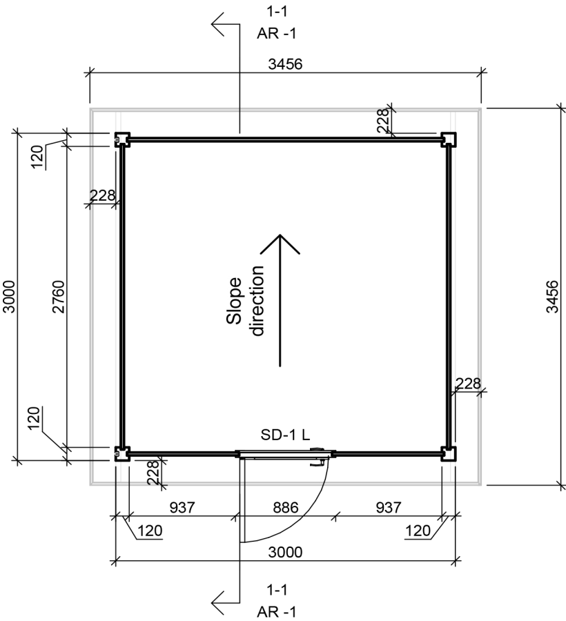
FLOOR PLAN
