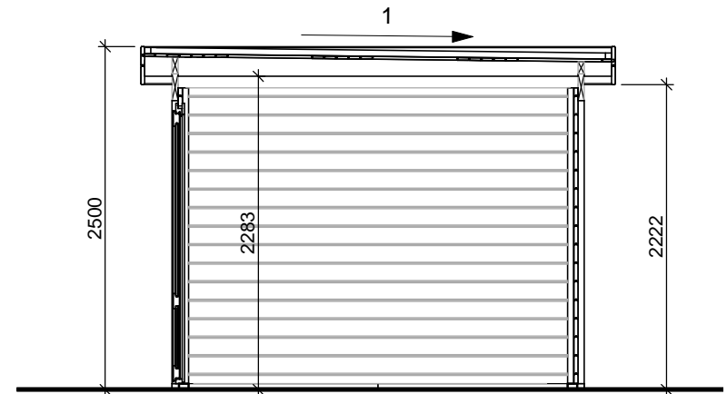
SECTION 1-1
