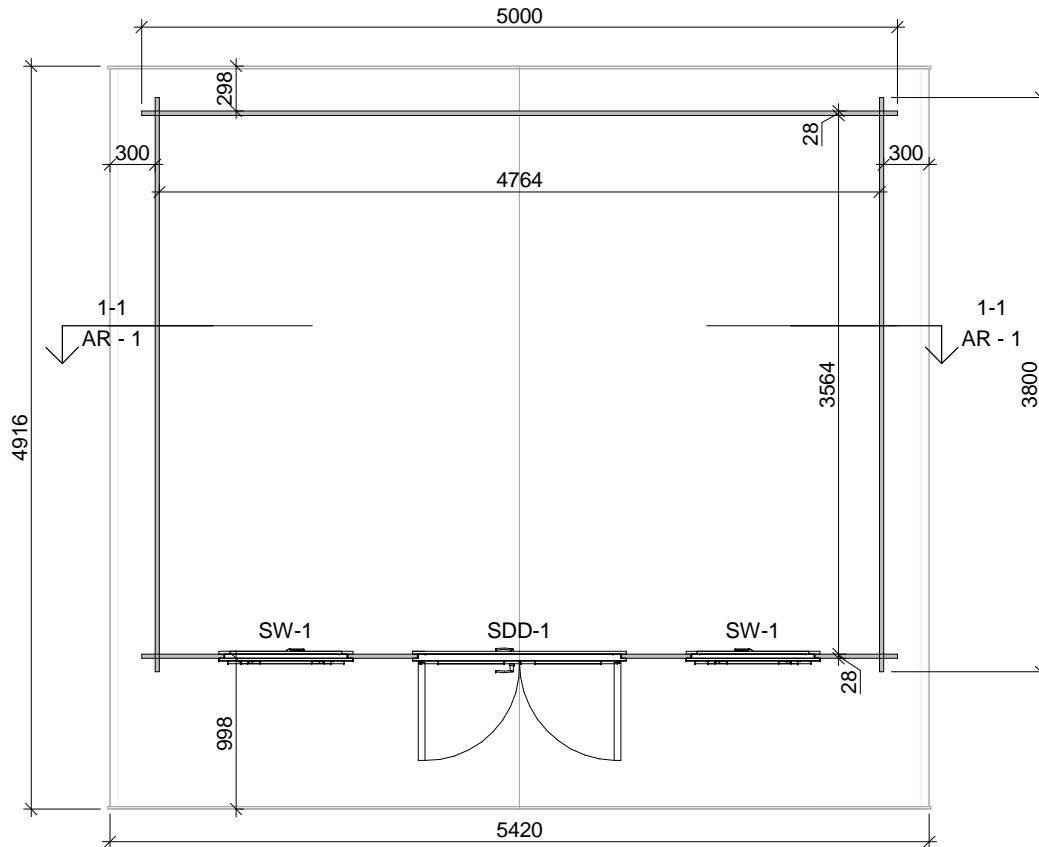
FLOOR PLAN
