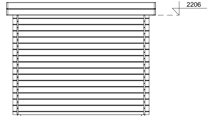
SECTION 1-1
