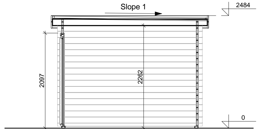
SECTION 1-1
