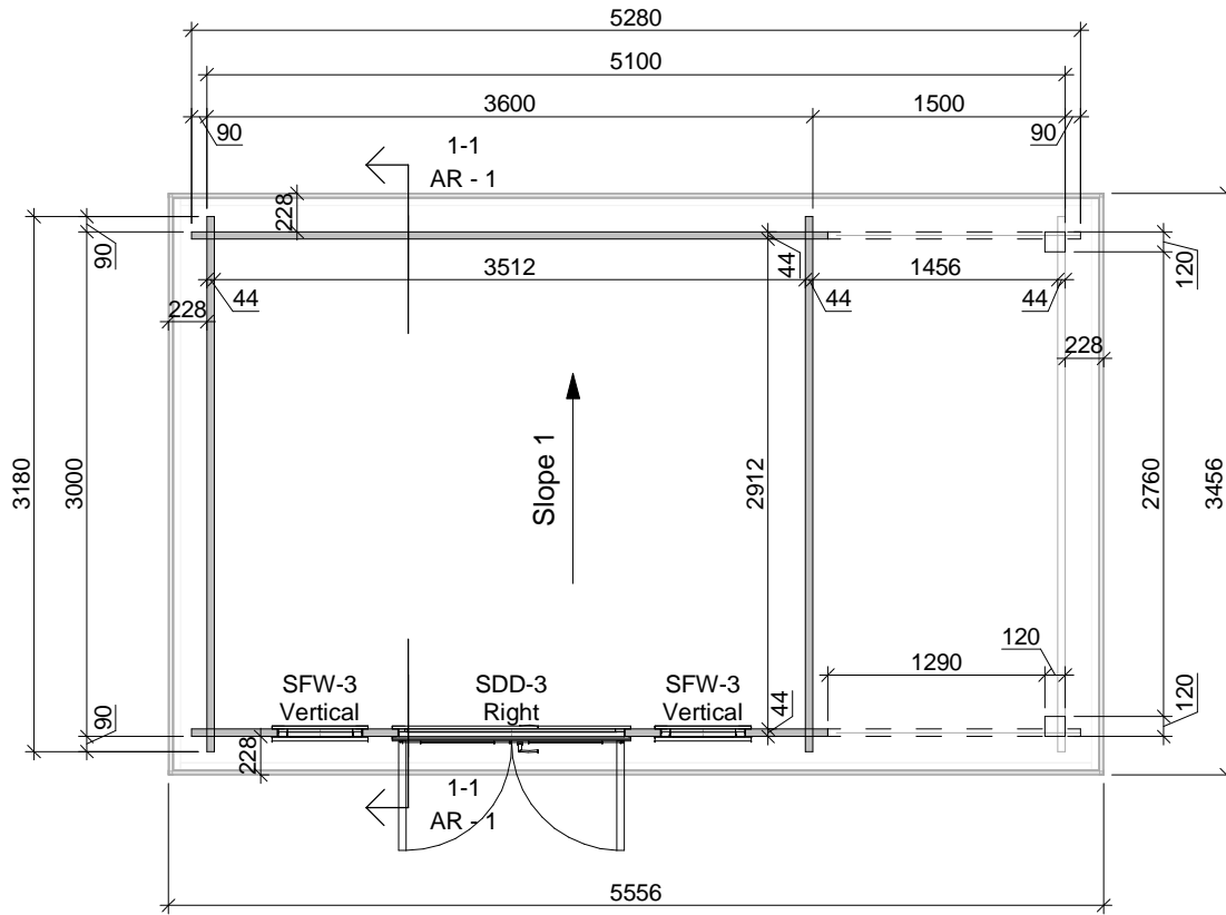
FLOOR PLAN
