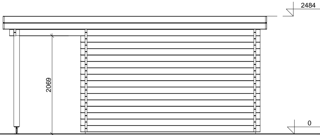
REAR VIEW
