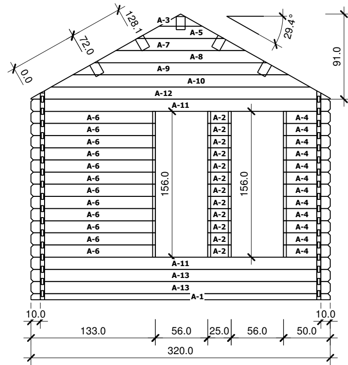
Gegnes 9,5x14,0
