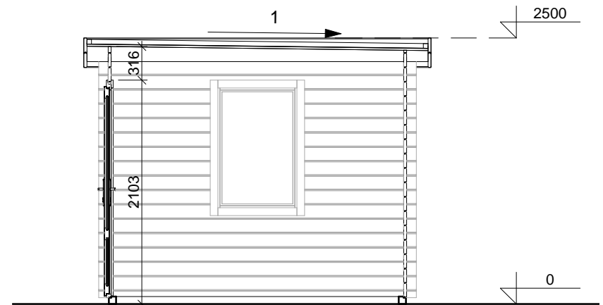
SECTION 1-1
