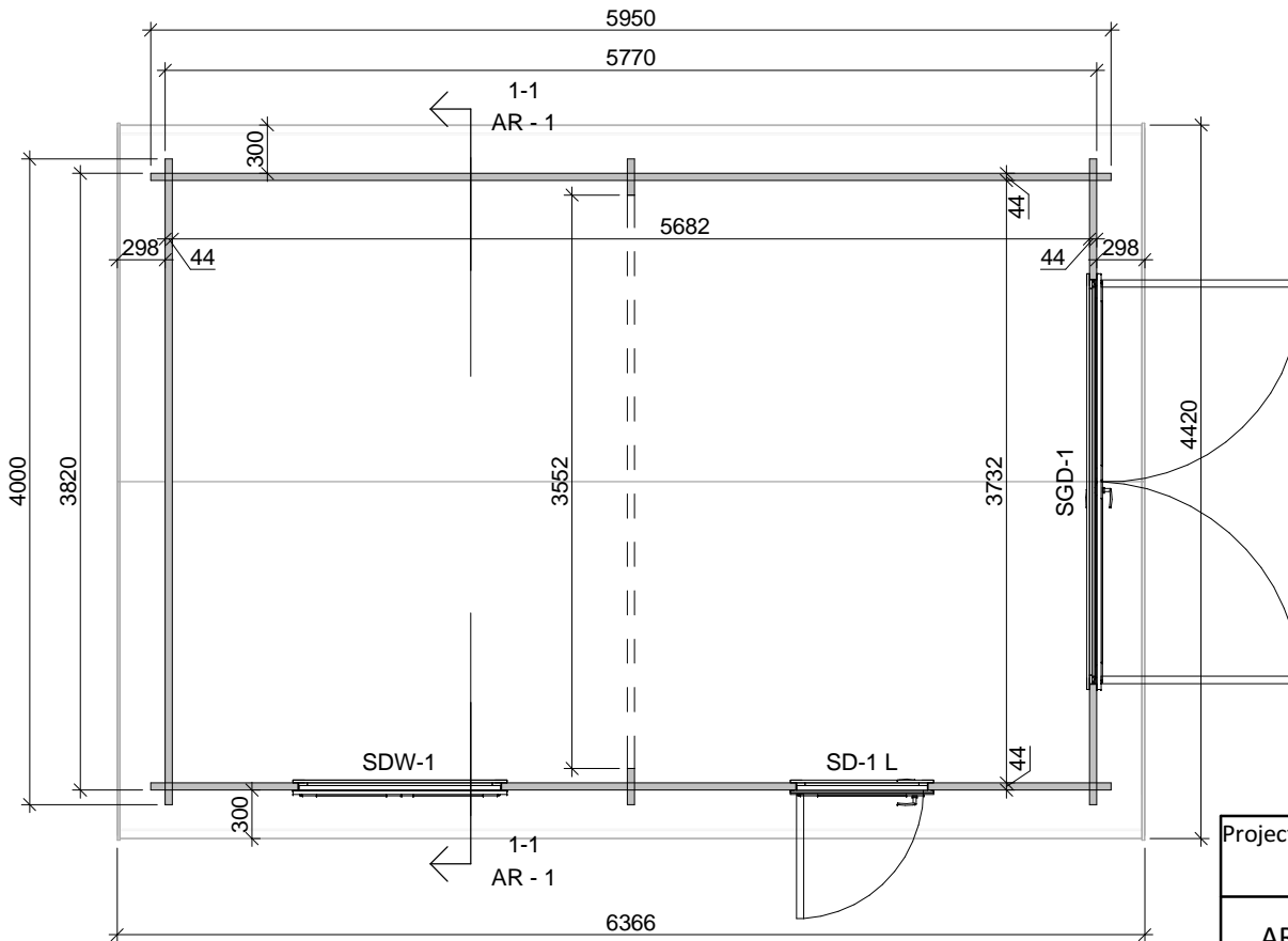
FLOOR PLAN
