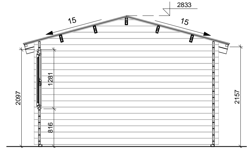
SECTION 1-1
