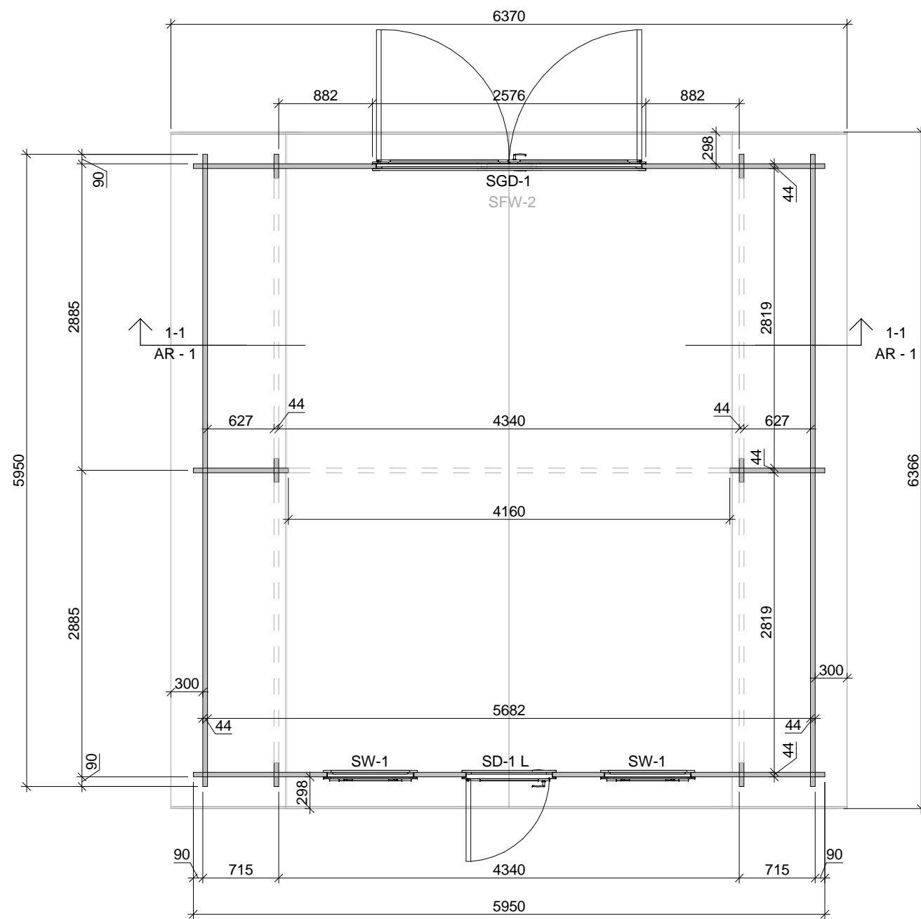
FLOOR PLAN
