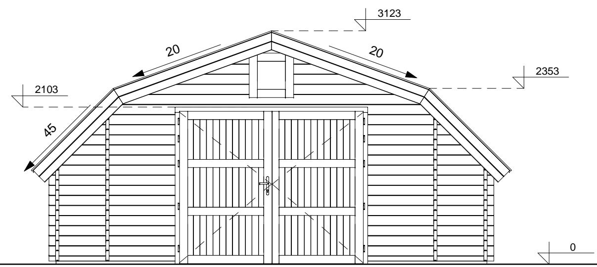
REAR VIEW
