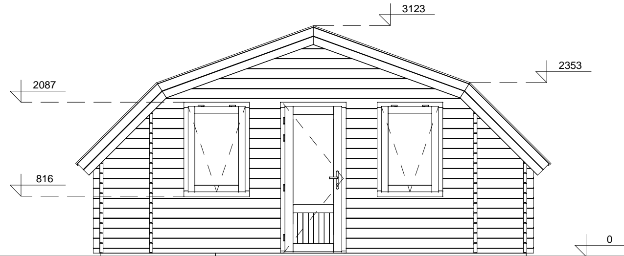
FRONT VIEW
