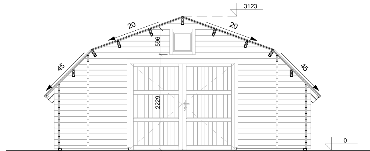
SECTION 1-1
