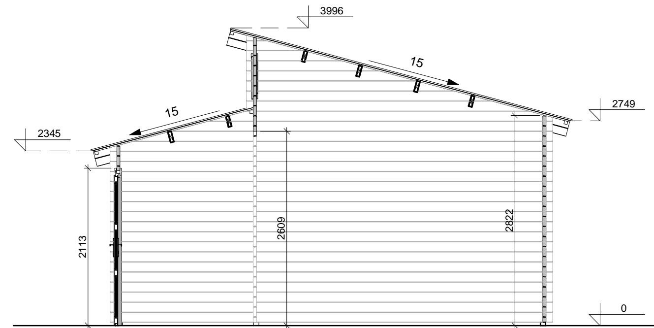
SECTION 1-1
