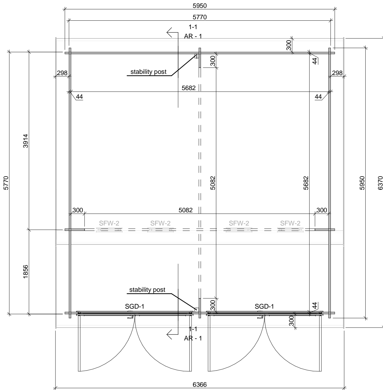
FLOOR PLAN
