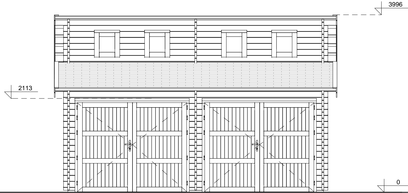
FRONT VIEW
